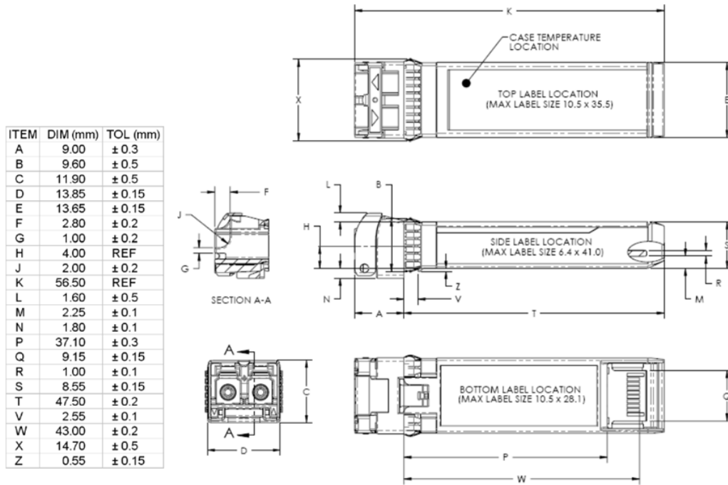
Figure 2. Mechanical Dimensions
