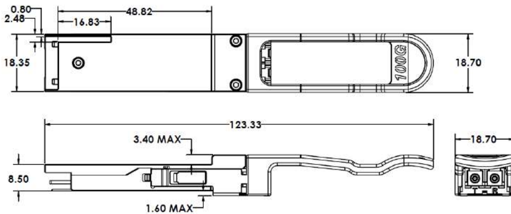
Figure 2. FTLC1156RDPL Mechanical Dimensions
