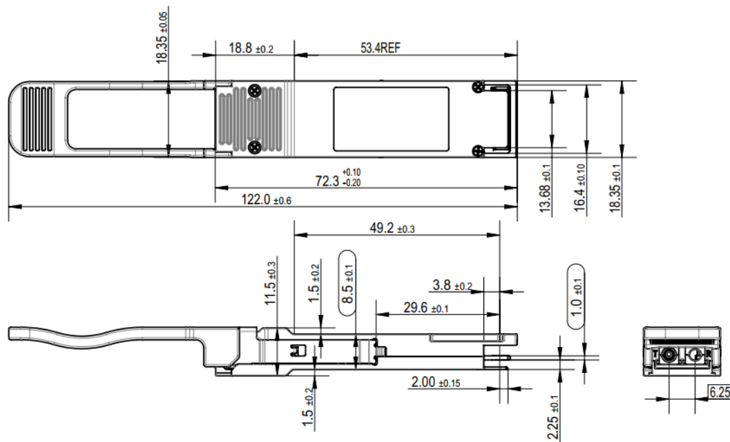
Figure 2. FTLC1159RGPL Mechanical Dimensions.
